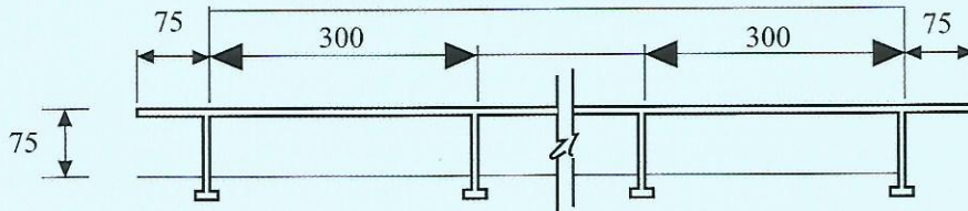
Anchor Layout For Curb Angle
