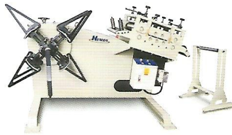
HLA 二機一體材料架 2 in 1 Uncoiler & Straightener
